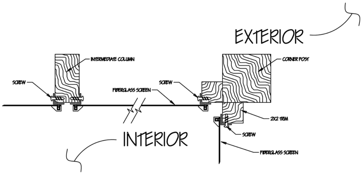
CORNER MOUNT INTERIOR DETAIL
