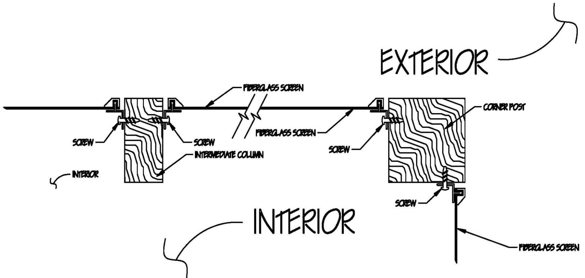
FLUSH MOUNT EXTERIOR DETAIL
