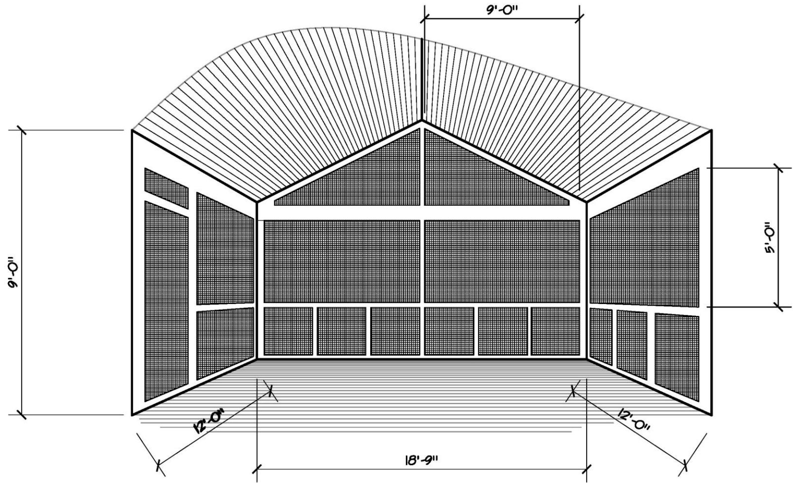
18'9" x 12' SCREEN PATIO
