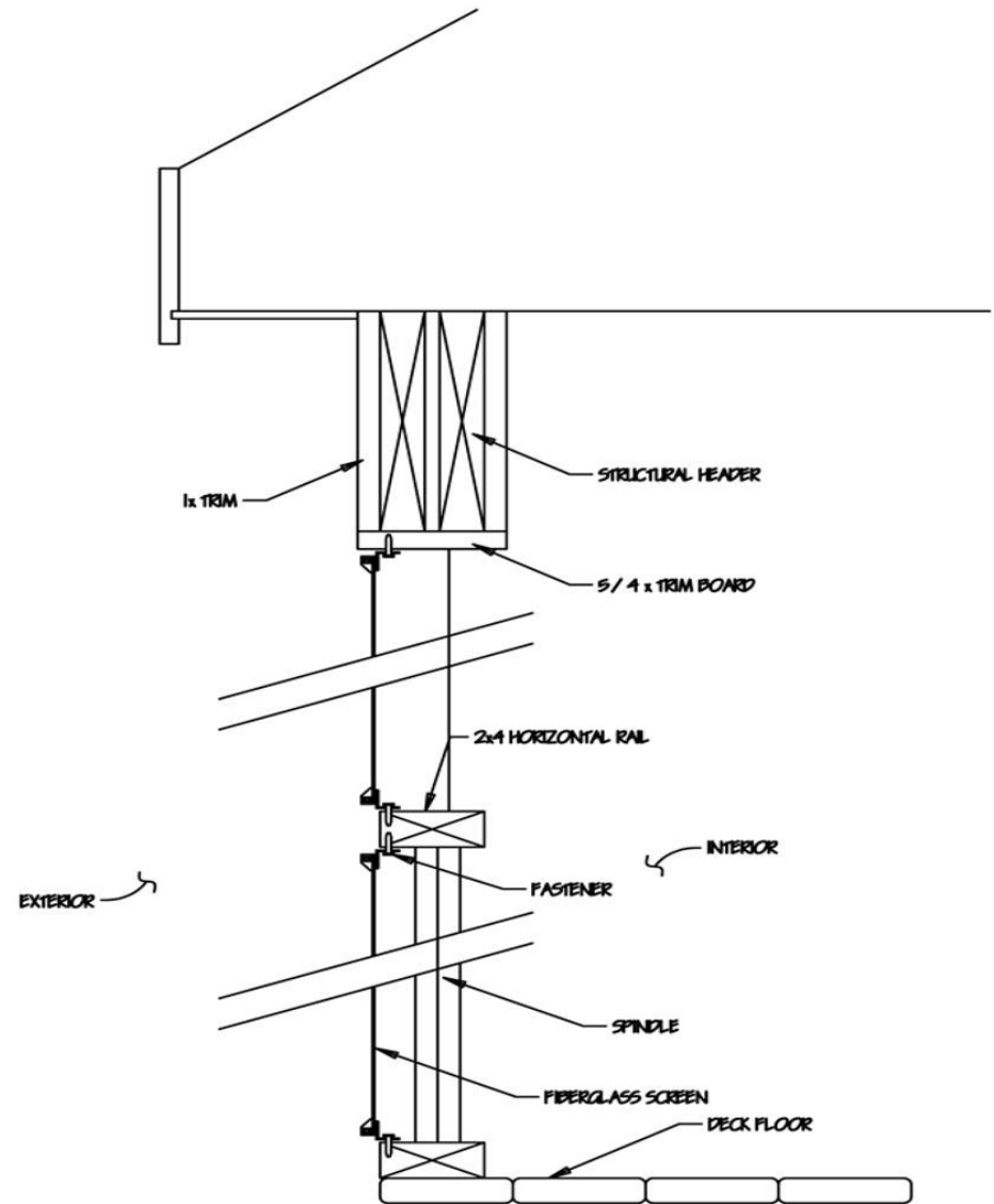
VERTICAL FLUSH MOUNT EXTERIOR DETAIL
