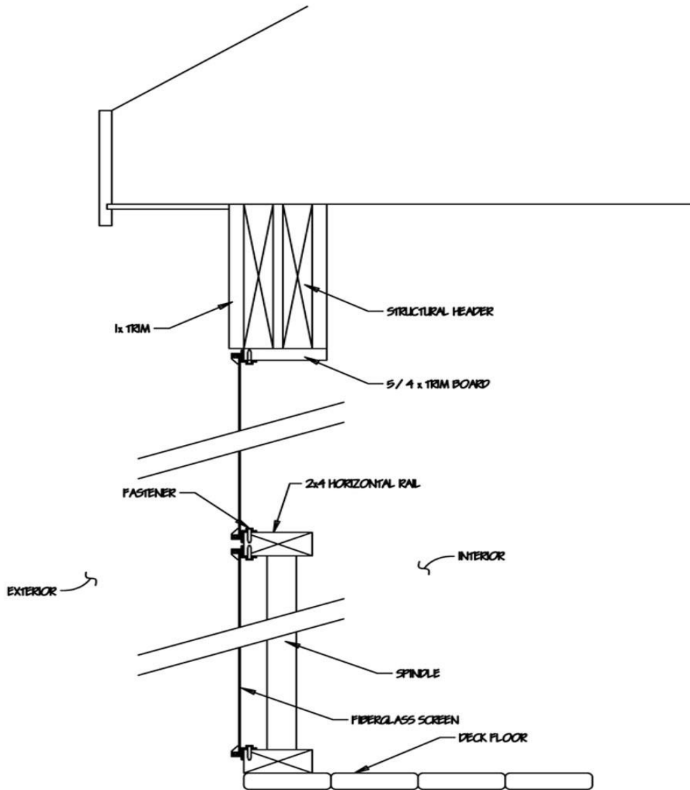
VERTICAL CORNER MOUNT EXTERIOR DETAIL
